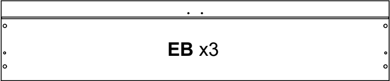
913x189x15mm
