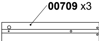
450x88x12,2mm
