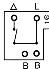
Wiring diagram
