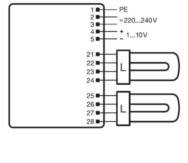
Wiring diagram
